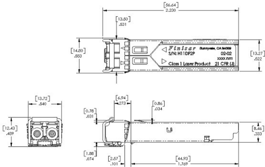
FWLF1524P2Vxx Outline Drawing
