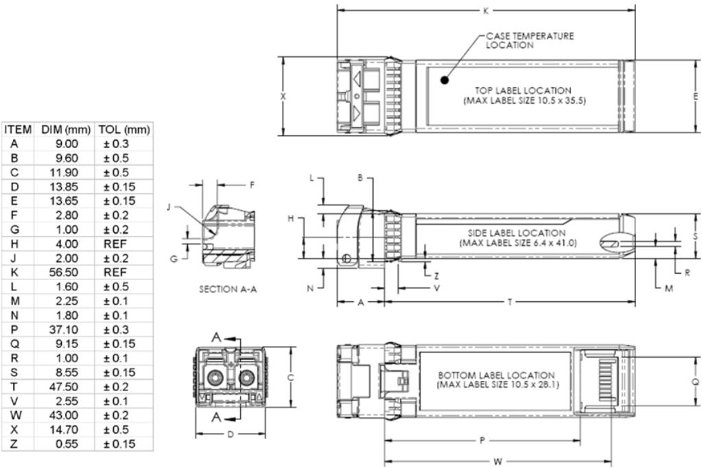
Figure 2. Mechanical Dimensions
