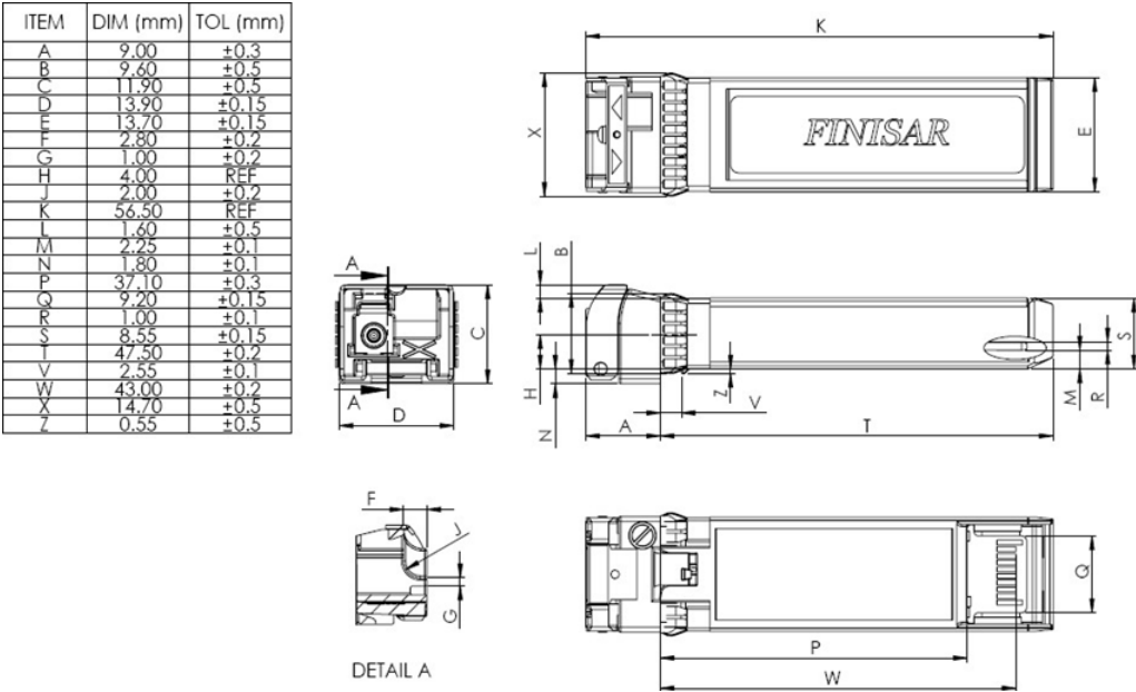
Figure 2. FTLX2072D327/FTLX2072D333 Mechanical Dimensions
