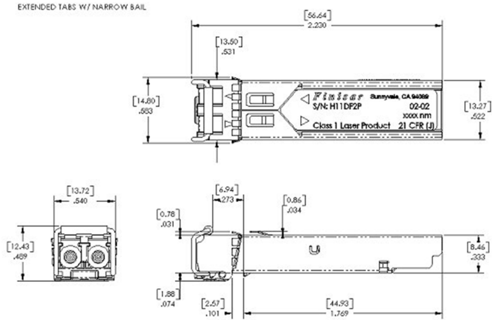
FTLF1321P1BTL
