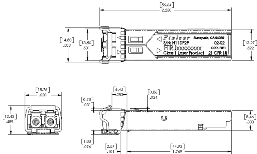
FTLF1321P1WTL
