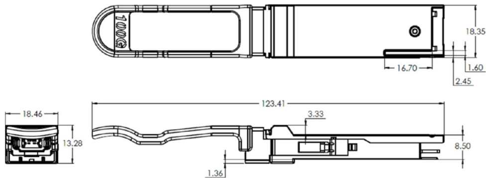
Figure 2. FTLC9555REPM Mechanical Dimensions.
