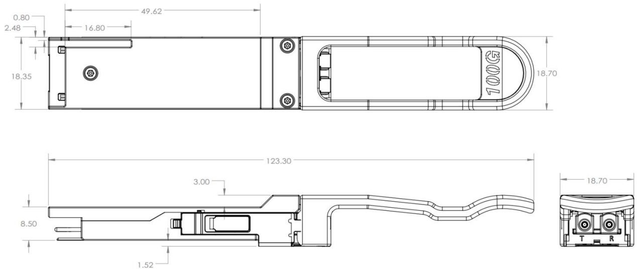
Figure 2. FTLC1156RDPL Mechanical Dimensions
