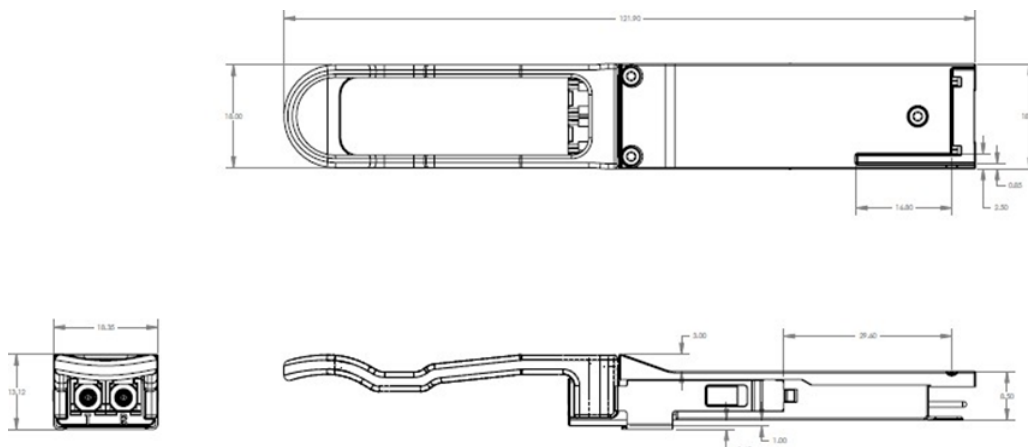
Figure 2 – FTL4E1QM1C mechanical drawing
