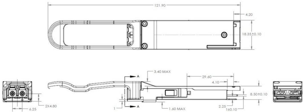
Figure 2 – FTL4C3QE2C mechanical drawing.
