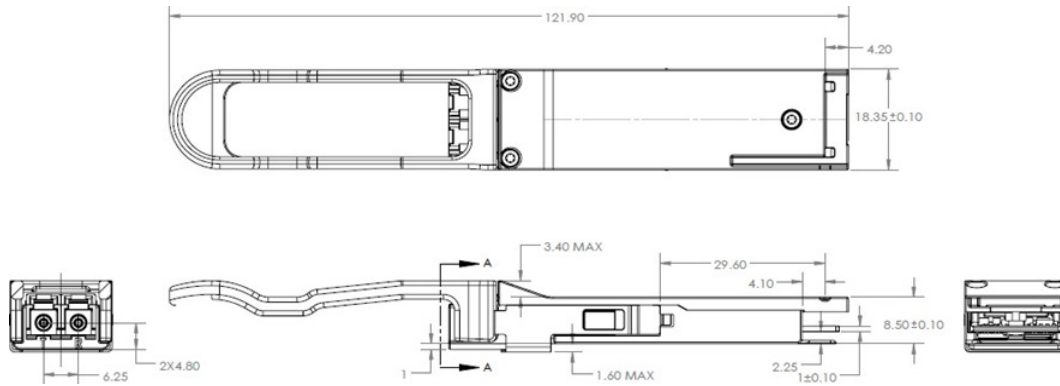
Figure 2 – FTL4C1QE2C mechanical drawing
