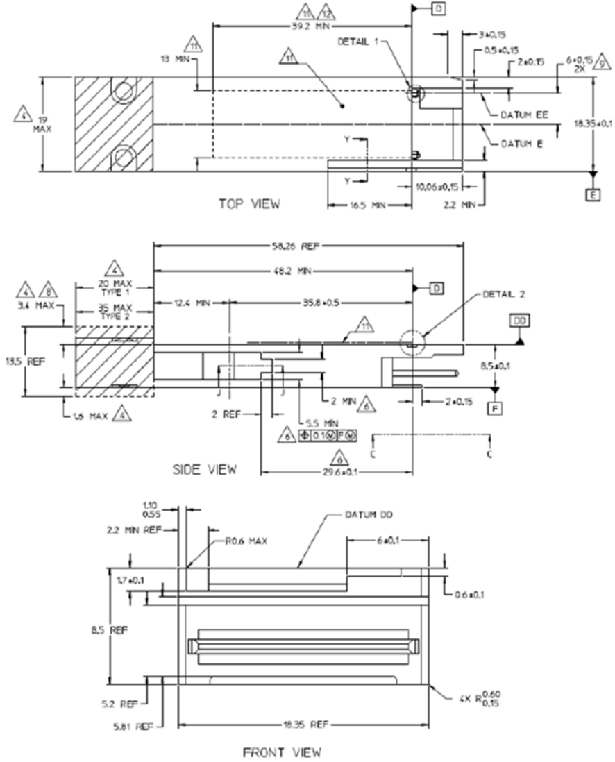
Figure 2. FTCD4533E2PxM Mechanical Dimensions.
