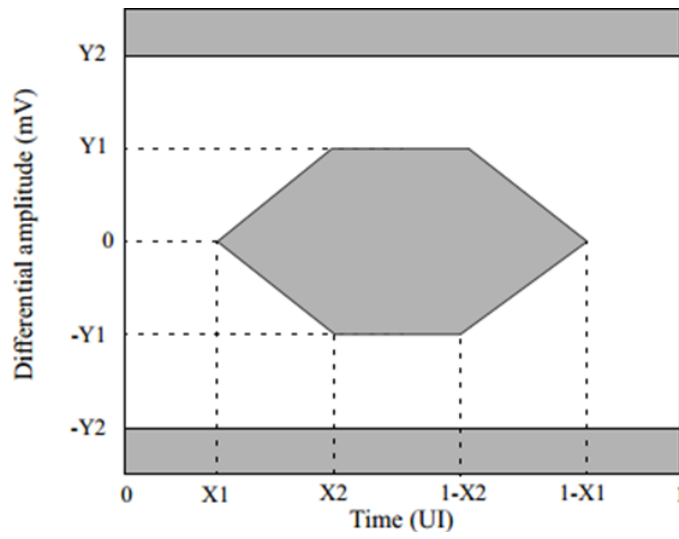
Figure 2 – Transmitter Input Differential Signal Mask
