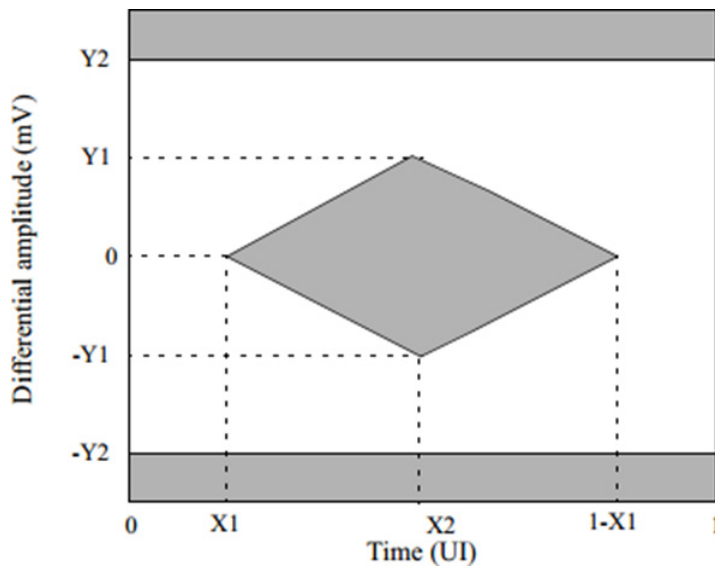
Figure 3 – Receiver Output Differential Signal Mask
