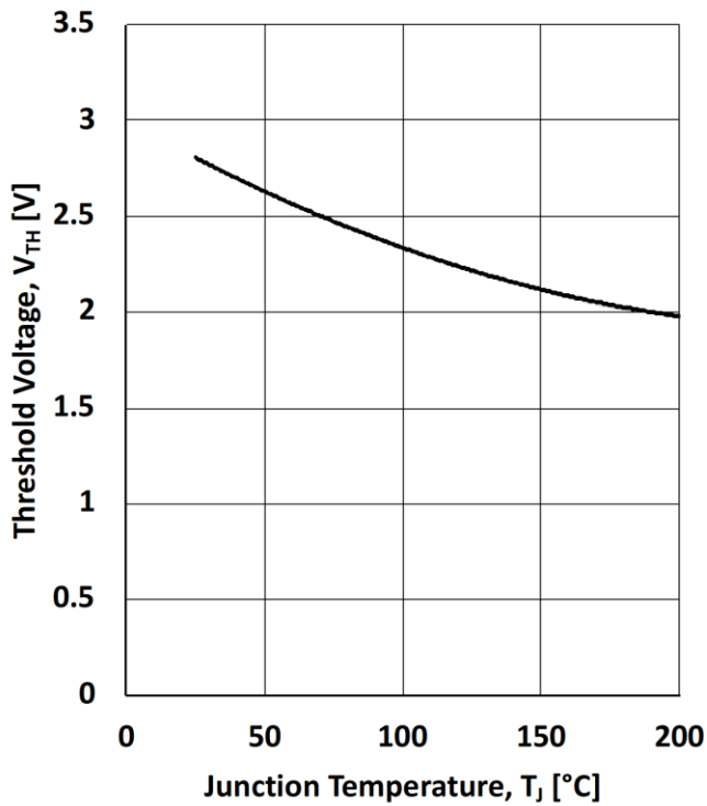
Figure 3. Threshold Voltage
