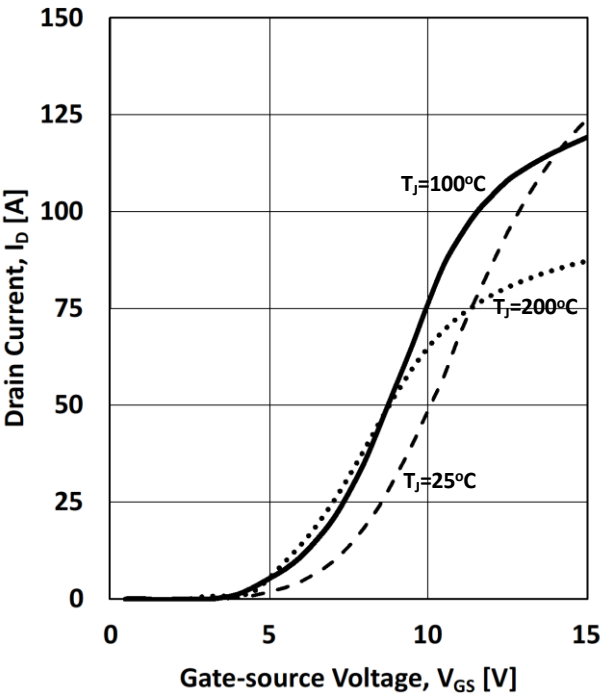
Figure 13. Transfer Characteristic I_D = f(V_{GS}); V_{DS} = 10 \text{ V};
