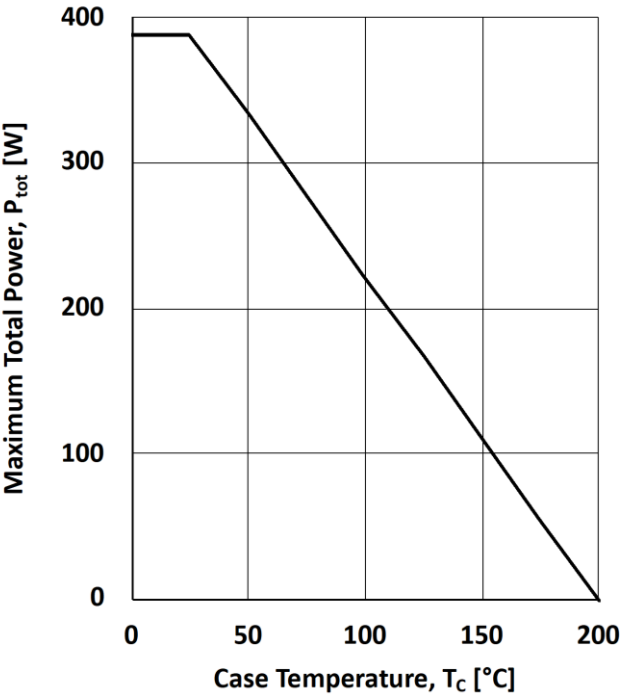
Figure 14. Power Dissipation P_{tot} = f(T_C)
