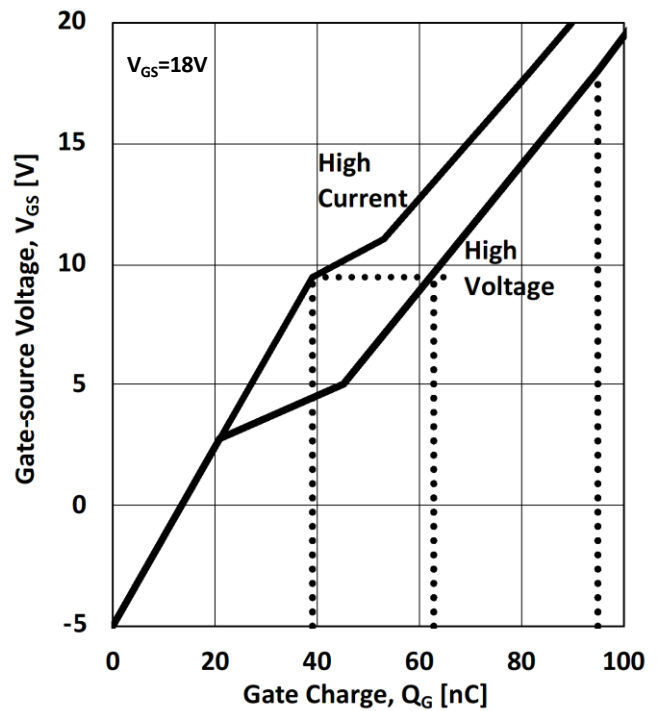
Figure 12. Gate Charge V_{GS} = (-5 \dots +18 \text{ V}) ; V_{DS} = 900 \text{ V} ; I_{DS} = 30 \text{ A} ; T_J = 25^\circ\text{C}
