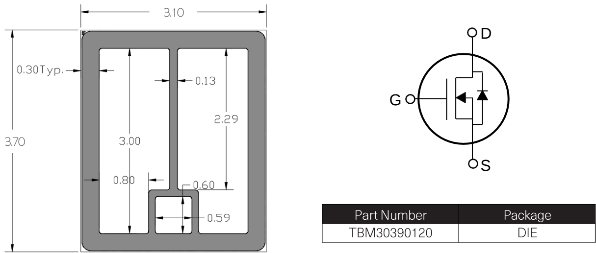
Figure 19. Chip Dimensions (mm) 5)
