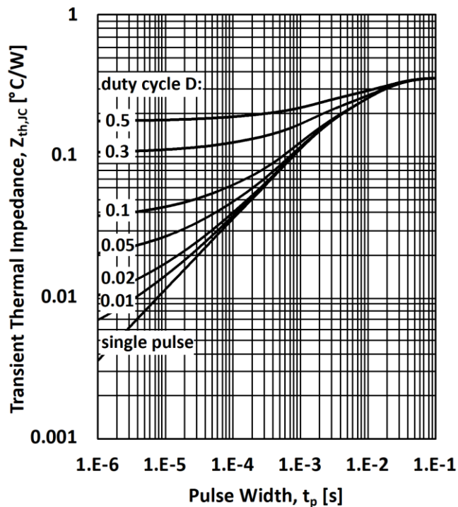
Figure 15. Transient Thermal Impedance Z_{thJC} = f(t_p, D); D = t_p / (\text{period})
