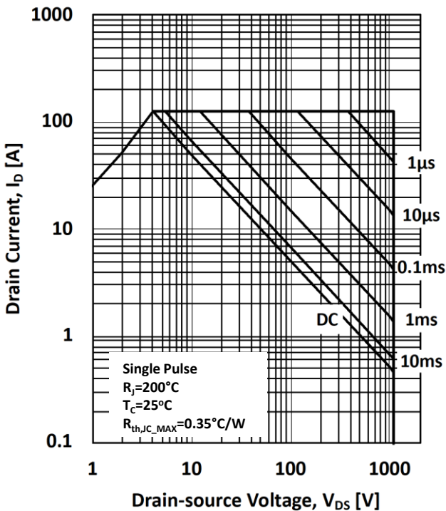
Figure 16. Safe Operating Area I_D = f(V_{DS}, t_p); T_C = 25^\circ\text{C}; D = 0 (Single pulse)
