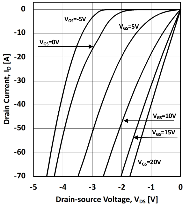
Figure 7. Third quadrant characteristics I_D = f(V_{DS}, V_{GS}); T_j = 25^\circ\text{C}
