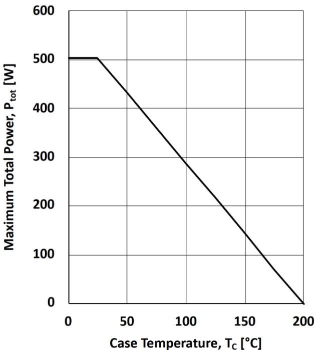
Figure 14. Power Dissipation P_{tot} = f(T_C)
