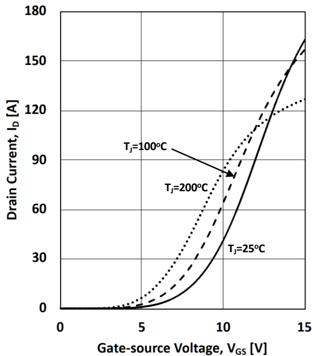
Figure 13. Transfer Characteristic I_D = f(V_{GS}); V_{DS} = 10\text{ V};
