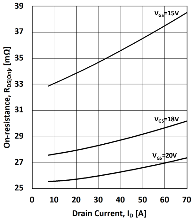
Figure 5. Drain-source on-state resistance R_{DS(on)} = f(I_D); T_j = 25^\circ\text{C}
