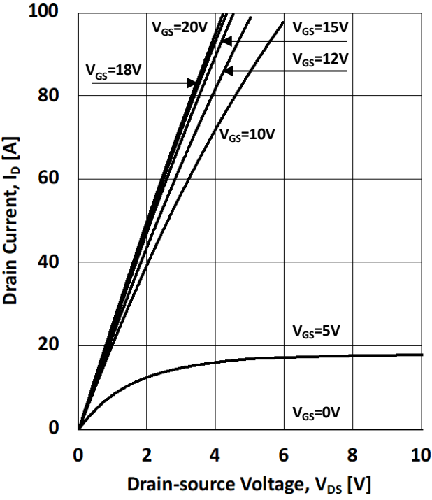
Figure 2. Output Characteristics I_D = f(V_{DS}, V_{GS}); T_J = 200^\circ\text{C}
