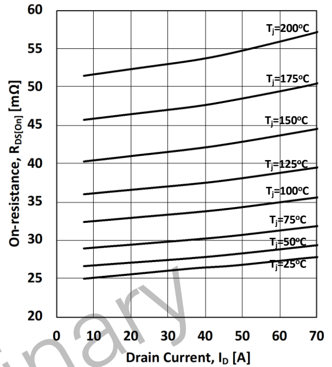
Figure 6. Drain-source on-state resistance
