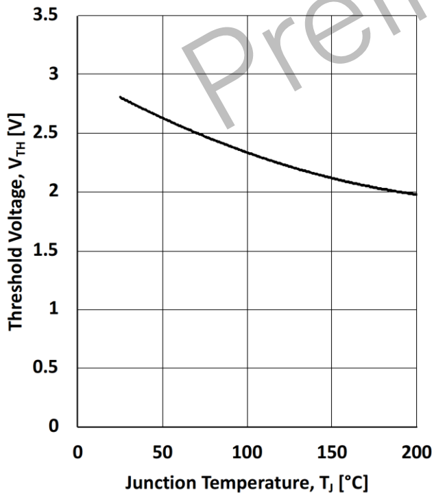
Figure 3. Threshold voltage V_{th} = f(T_J); V_{DS} = V_{GS}; I_D = 13 \text{ mA}
