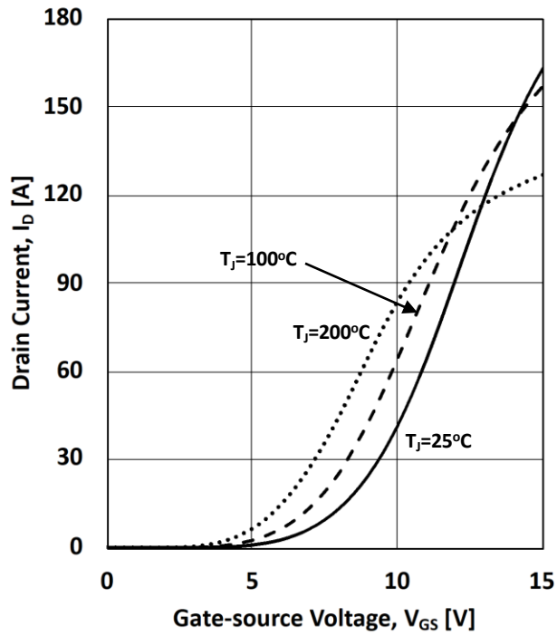
Figure 13. Transfer Characteristic
