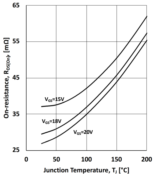
Figure 4. Drain-source on-state resistance R_{DS(on)} = f(T_J); I_D = 55 \text{ A}
