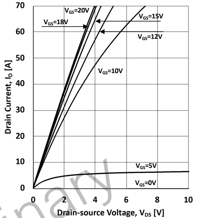
Figure 2. Output characteristics I_D = f(V_{DS}, V_{GS}); T_J = 200^\circ\text{C}
