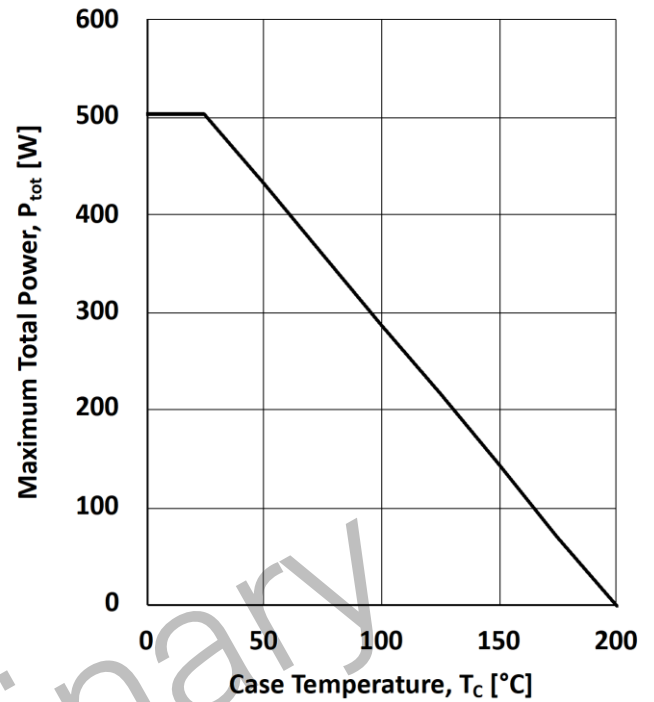
Figure 14. Power Dissipation
