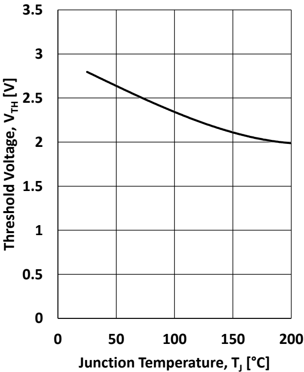
Figure 3. Threshold voltage
