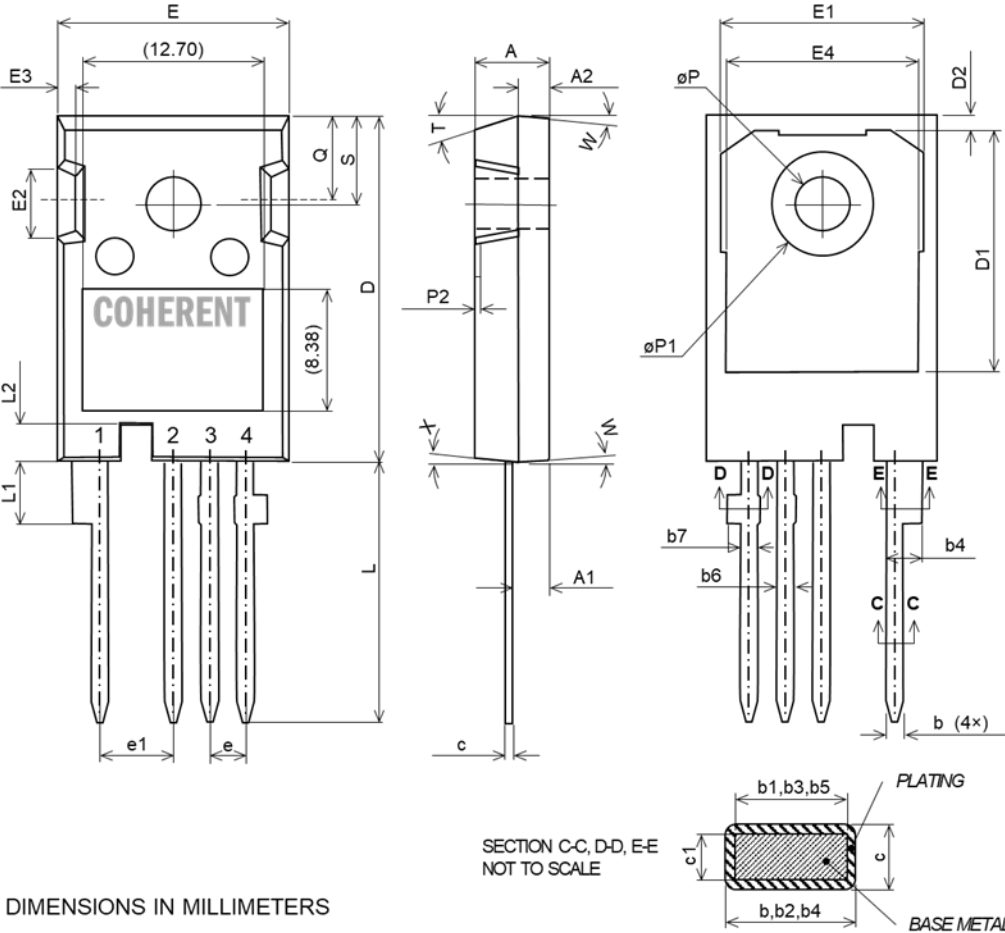
Figure 19. Part Dimensions (mm)
