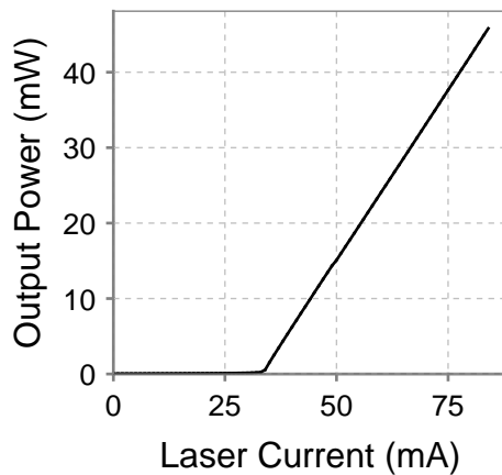
Output Power vs. Forward Current (40 degC)
