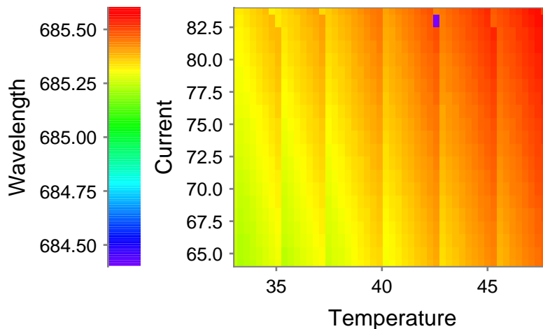
Current (mA), Temperature (degC), Wavelength (nm)
