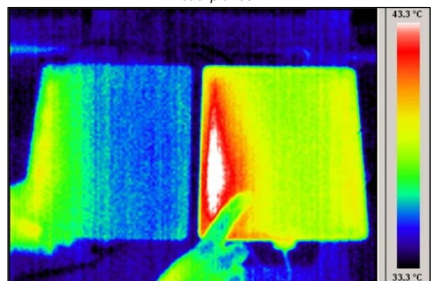
Thermal comparison of iPad2 and iPad3 both based on a-Si backplanes
