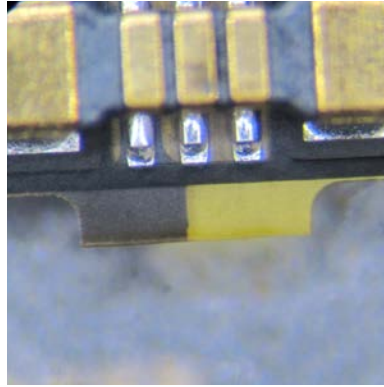
Cutting edge of PCB
