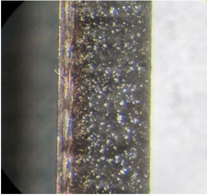
Cross-section of laser-cut PCB
