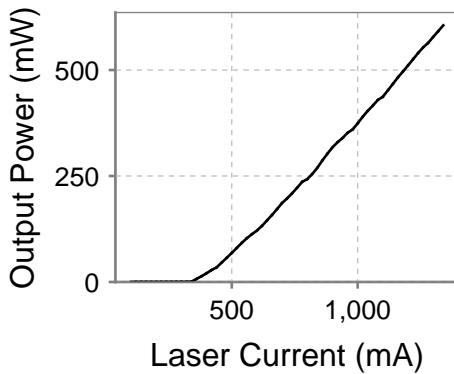
Output Power vs Forward Current
