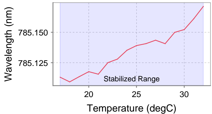
Wavelength vs. Temperature
