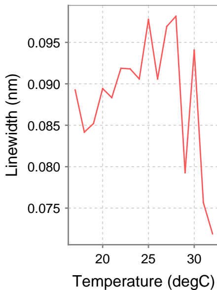
Linewidth vs. Temperature
