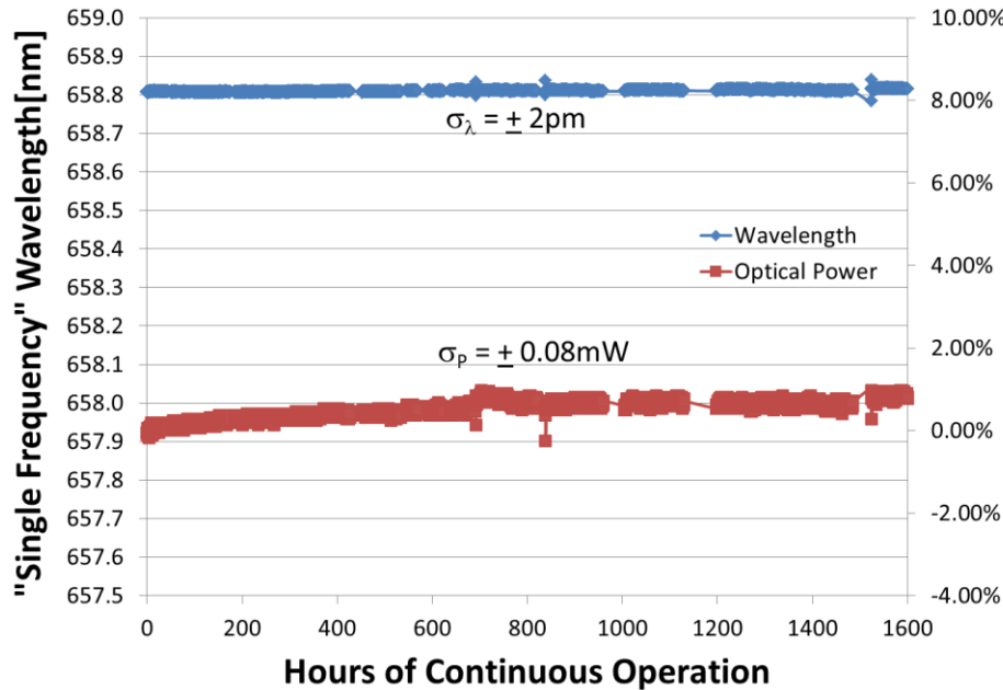
Ondax 35mW 658nm Laser Stability X4129
