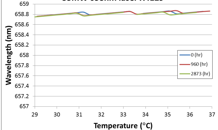
35mW 658nm laser X4129
