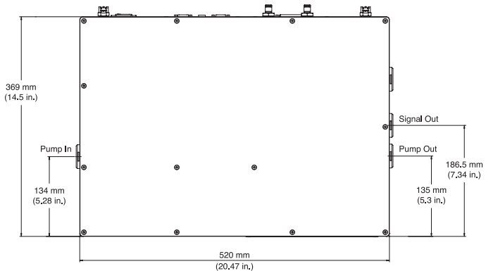
Chameleon MPX - Side View
